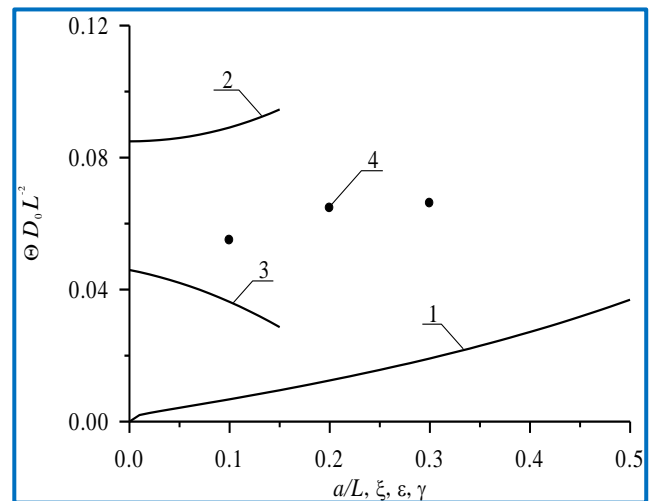
Fig.7. Dependences of dimensionless optimal annealing time for doping by ion implantation, which have been obtained by minimization of mean-squared error, on several parameters. Curve 1 is the dependence of dimensionless optimal annealing time on the relation a/L and \xi = \gamma = 0 for equal to each other values of dopant diffusion coefficient in all parts of heterostructure. Curve 2 is the dependence of dimensionless optimal annealing time on value of parameter \varepsilon for a/L=1/2 and \xi = \gamma = 0 . Curve 3 is the dependence of dimensionless optimal annealing time on value of parameter \xi for a/L=1/2 and \varepsilon = \gamma = 0 . Curve 4 is the dependence of dimensionless optimal annealing time on value of parameter \gamma for a/L=1/2 and \varepsilon = \xi = 0
