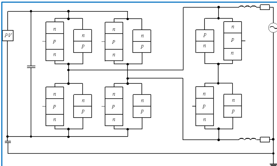
Fig.1a. Structure of the considered inverter [15]
