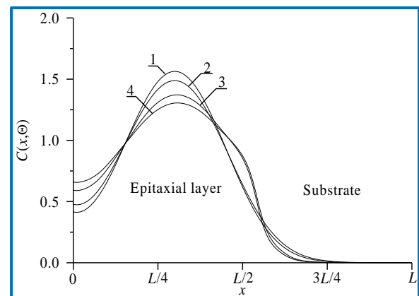
Fig 2b. Dependences of concentration of dopant, implanted in heterostructure from Figs. 1, on coordinate in
