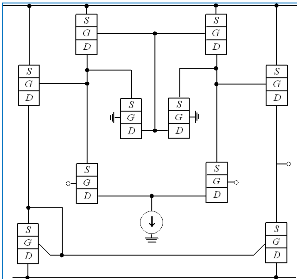
Fig 1. The considered limiting amplifier circuit [4]
