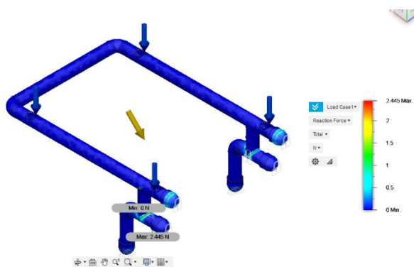
Fig. 4 Reaction Force
