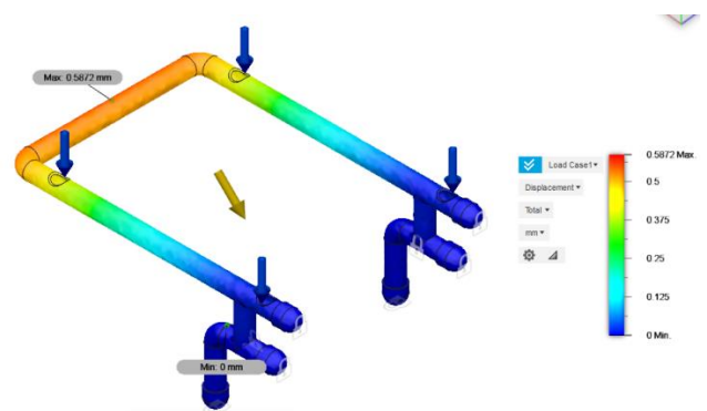
Fig. 3 Displacement Diagram
