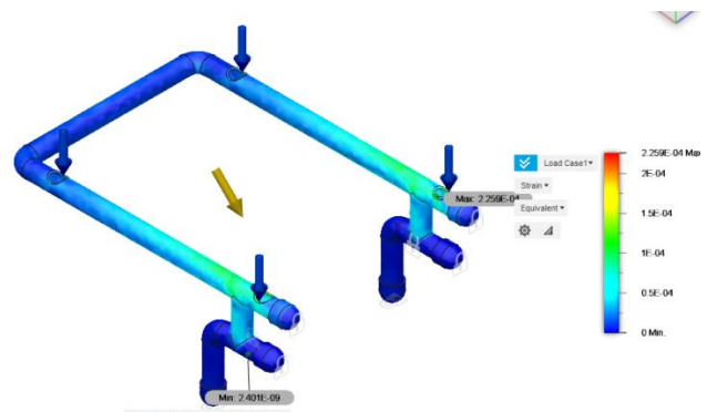
Fig. 2 Strain Analysis
