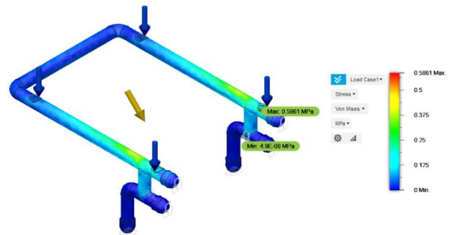
Fig. 1 Stress Analysis
