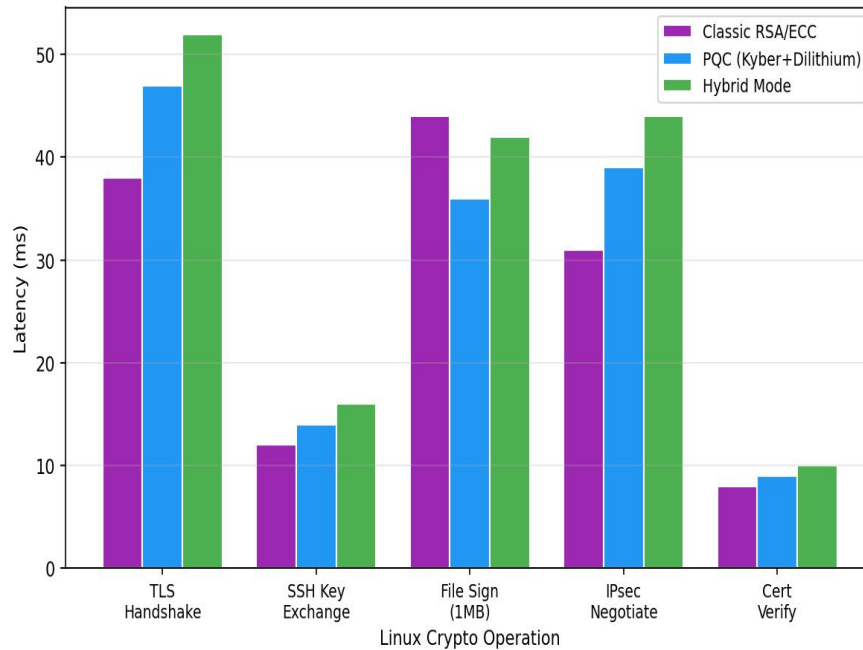
Figure 1: Cryptographic overhead comparison on enterprise Linux (RHEL 9)
